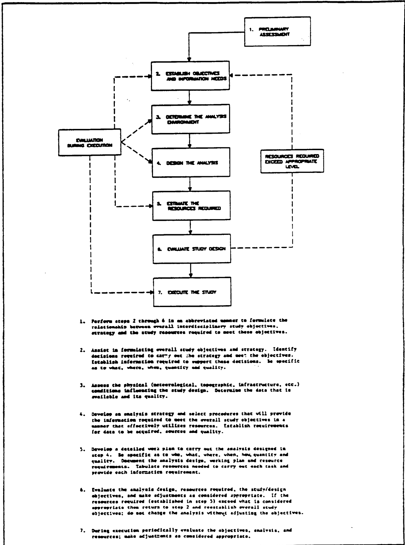
FIGURE 3.1 Hydrologic Study Design
